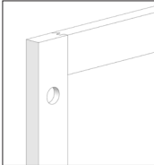
Concealed Kitchen Hinge Drilling
